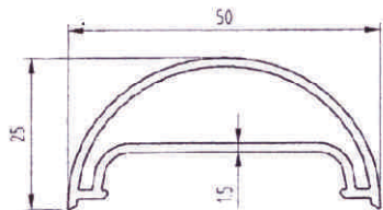
PROTECTING PROFILE
