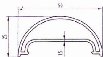
PROTECTING PROFILE
