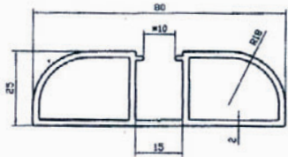
PROTECTING PROFILE
