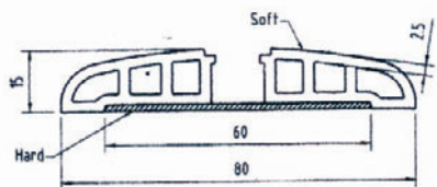
PROTECTING PROFILE
